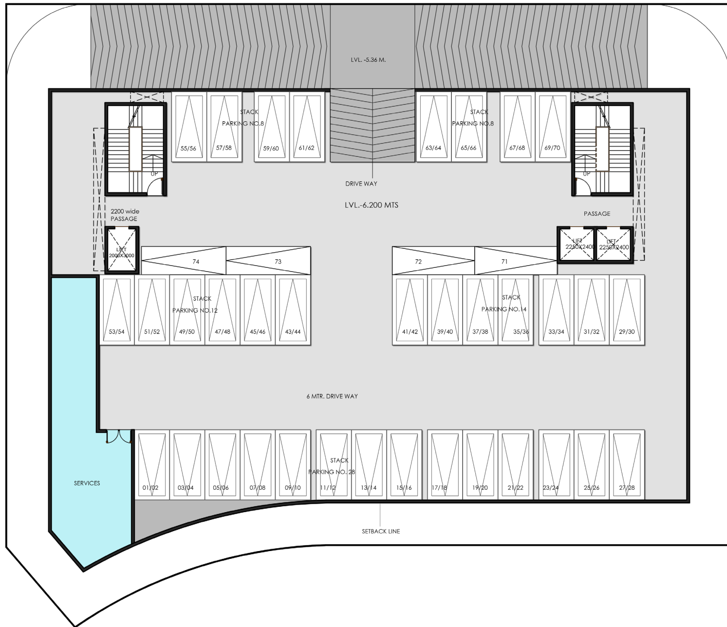
BASEMENT PLAN
